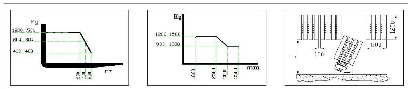
Diagram of maximum loads regarding the lifts.
